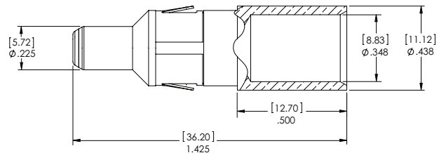
ITA Contact, Part # 610 150 101
